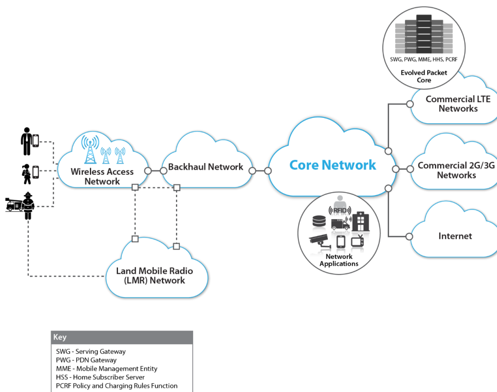
Figure 5.1.1-2: Wireless Network Configuration
